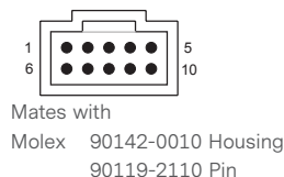
Figure 2. Connector J1
