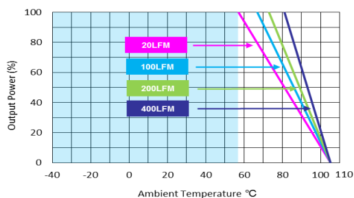
MJW25-24S033, MJW25-48S033 Derating Curve without Heatsink
