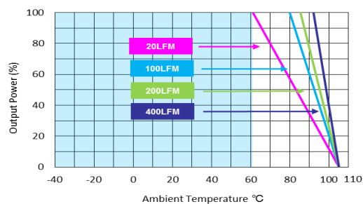
MJW25-12S033 Derating Curve with Heatsink
