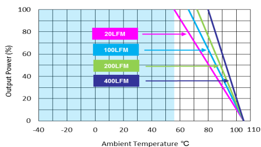
MJW25-24S05, MJW25-24S12, MJW25-24S15, MJW25-48S05 MJW25-48S12, MJW25-48S15 Derating Curve without Heatsink
