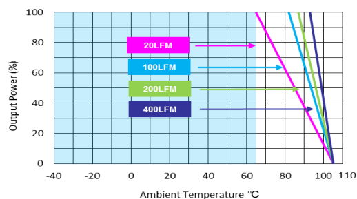
MJW25-24S033, MJW25-48S033 Derating Curve with Heatsink
