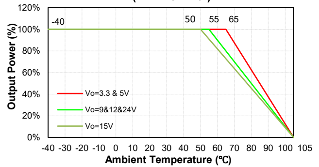
NCS01W8 Typical Derating Curve (Vin=Nominal)
