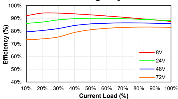
NCS01W8-48S050 Eff Vs Io @25 Deg. C
