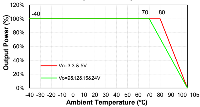
NCS01W8 Typical Derating Curve (Vin=Nominal)
