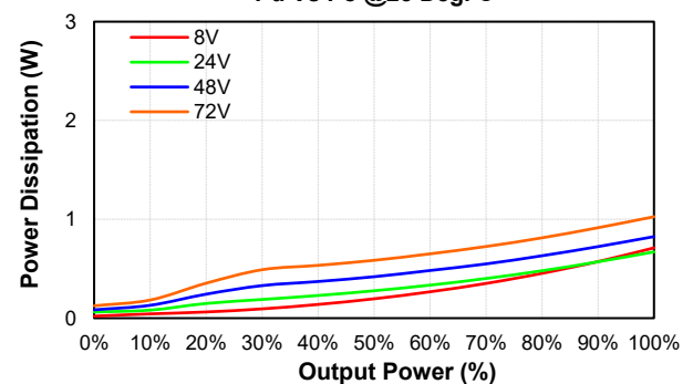
NCS01W8-48S050 Pd Vs Po @25 Deg. C
