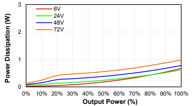
NCS01W8-48S033 Pd Vs Po @25 Deg. C
