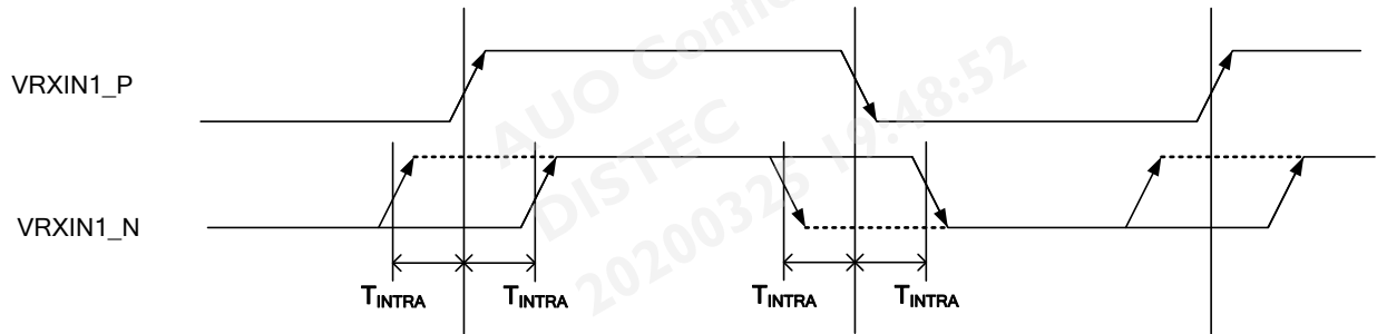
Note7. V-by-one Inter-pair Skew
